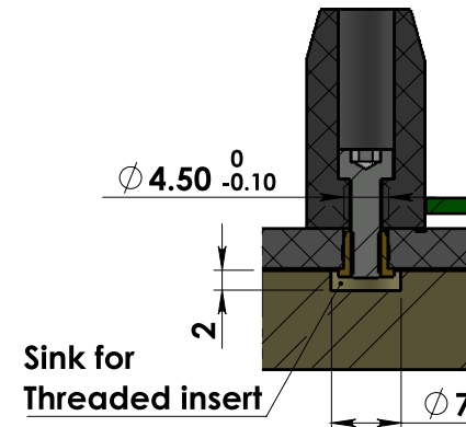
DETAIL C SCALE 1.2 : 1 Hole measures for Threaded inserts
