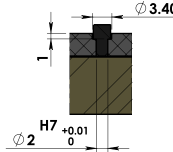
DETAIL B SCALE 1.5 : 1 Hole measures for PCB supports
