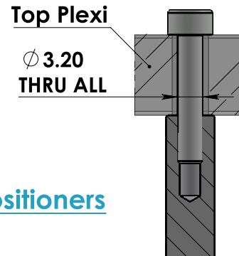
DETAIL D SCALE 1.5 : 1 Hole measure for Pushrod screws
