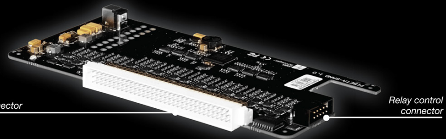
Standalone control connector
